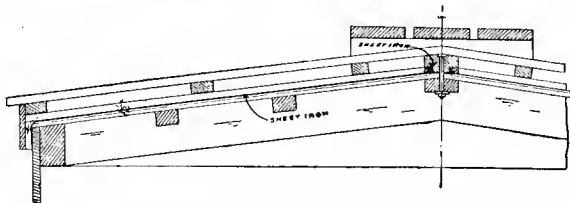
Fig. 2386. Transverse Section.
